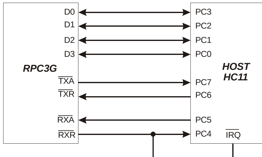
figure 17: RPC3G to HC11 \mu -C interface
