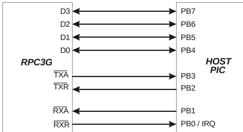
figure 16: RPC3G to PIC - \mu C interface
