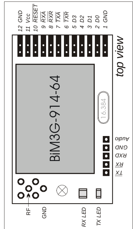
figure 4: RPC3G's pinout
