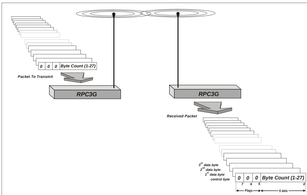
figure 6: RPC3G ↔ Host data transfer
